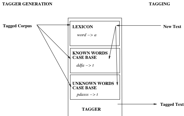
Figure 3: Architecture of the tagger-generator: flow of control.
