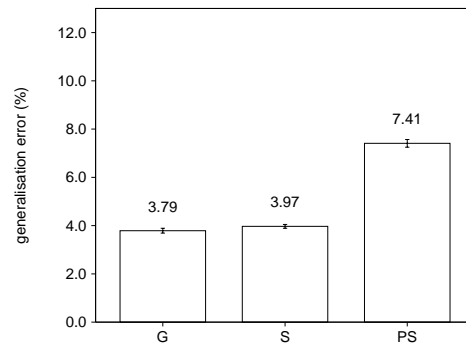
Figure 4: Percentage of generalisation errors made by IGTREE on the GS task, in terms of the percentage of incorrectly classified test instances as well as on phonemes and stress assignments computed separately.
