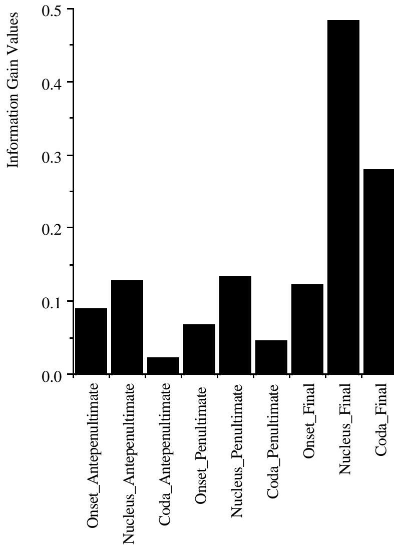
Figure 1: Information Gain Values for Dutch monomorphemes.
